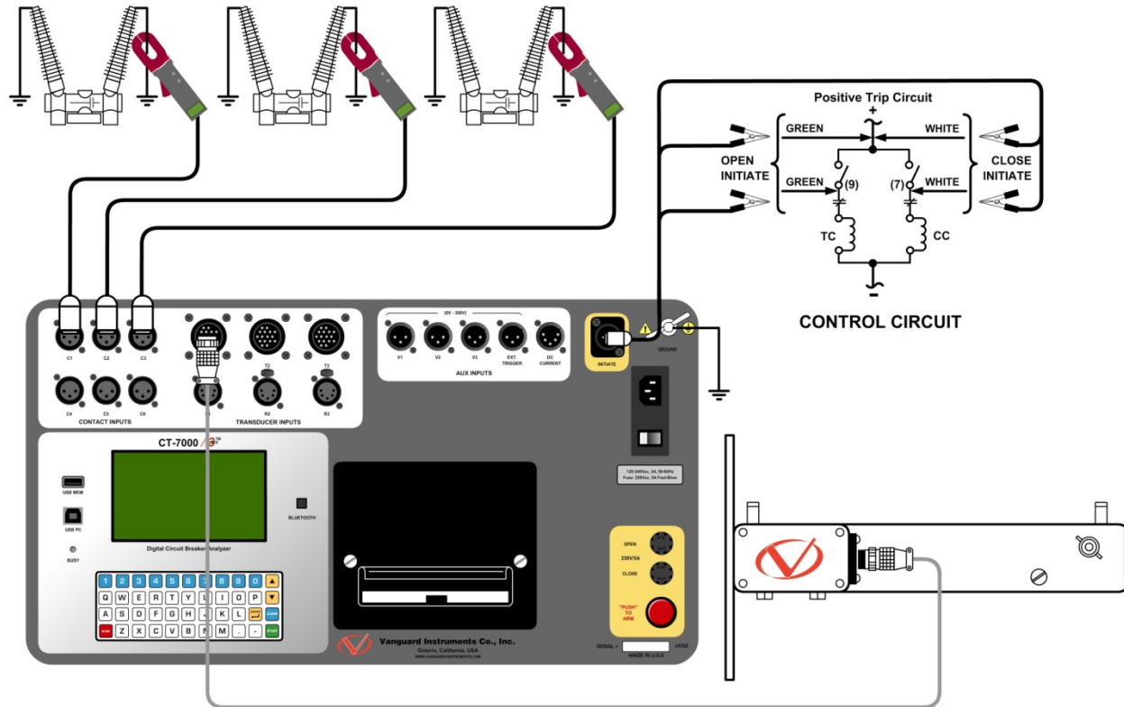
Dual Ground Timing Connections
